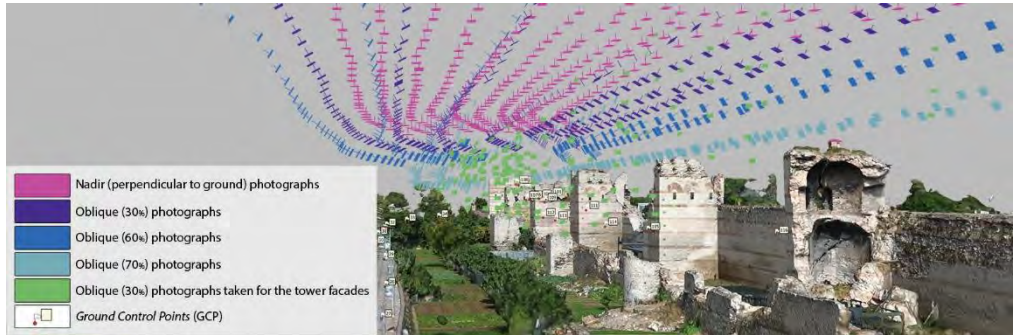
Fig. 5- Typical flight pattern for aerial acquisition (model view from the software)
