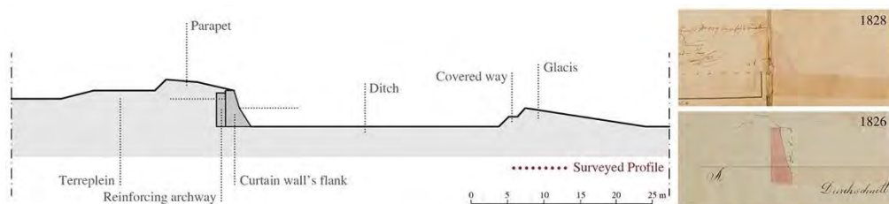
Fig. 7- Cross-section of the central bastion, shown alongside historical sectional drawings (graphic elaboration by Federico Panarotto, 2025)
