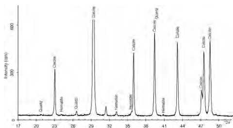
Fig. 7- XRD pattern
