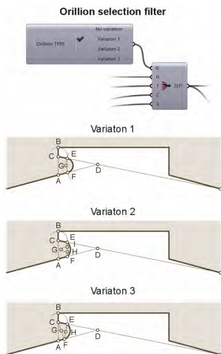
Fig. 4- Orillon variation and visual algorithm control nodes (graphic elaboration by F. Natta)
