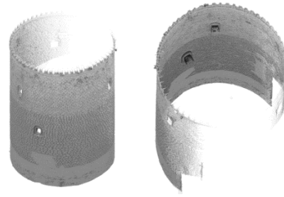
Fig. 4- Point cloud showing missing parts (graphic elaboration by the authors, 2025)
