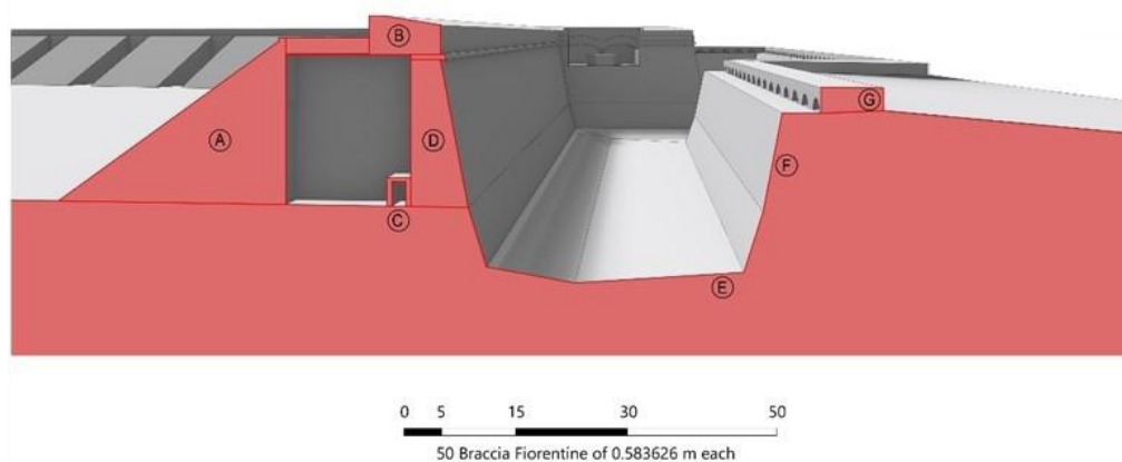
Fig. 4- Section of the fortified models: A) pomerium ; B) parapet; C) countermine; D) scarp; E) moat; F) counterscarp; G) covered way. Graphic scale in braccia fiorentine (graphic elaboration by Lorenzo Belli, 2025)
