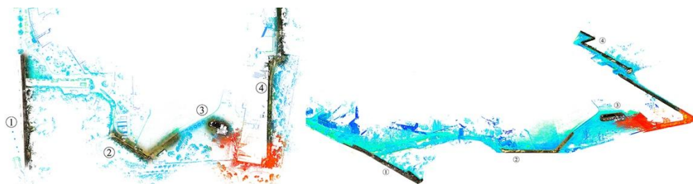
Fig. 4- Plan (left) and axonometric view (right) from the point cloud: 1) stone portal and SW curtain wall; 2) bastion on via Morandi; 3) modern building over SE bastion; 4) NE curtain wall, partly overbuilt (graphic elaboration by Gianlorenzo Dellabartola, 2025)
