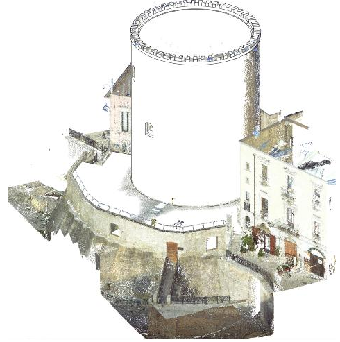
Fig. 9- Scan-to-BIM integration phase (graphic elaboration by the authors, 2025)
