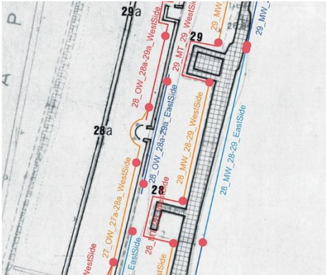
Fig. 7- A layout of close-range acquisition scenarios and distribution of telescopic measuring rods as scale bars
