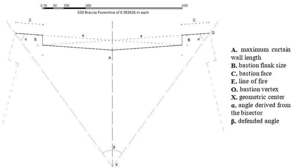
Fig. 2- Critical redrawing of the planimetric profiling scheme of fortifications referred to a generic defended angle. Graphic scale in braccia fiorentine (graphic elaboration by Lorenzo Belli, 2025)
