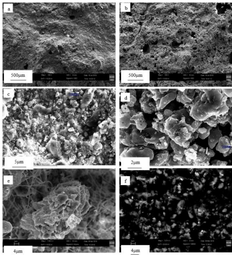
Fig. 8- SEM images and EDX spectra of: 'intonachino' (a); inner detachment surface with rounded pores (b); zoom on the surface sample (c); detail of internal fabric (d); organic filaments and microorganisms of the detachment surface (e); backscattered images showing iron oxides distribution (bright spots) in the sample matrix (f)
