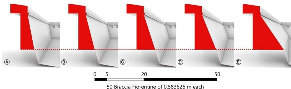
Fig. 5- Different scarp configurations described in the treatise (Maggi & Castriotto, 1564: Book II, Chap. I, fol.42 r.). Graphic scale in braccia fiorentine (graphic elaboration by Lorenzo Belli, 2025)
