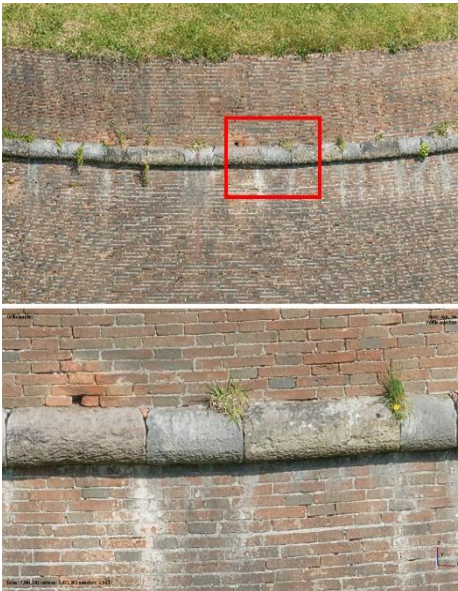
Fig. 3- Photogrammetric model of a detailed part of a bastion with close-up (source: authors' data processing)
