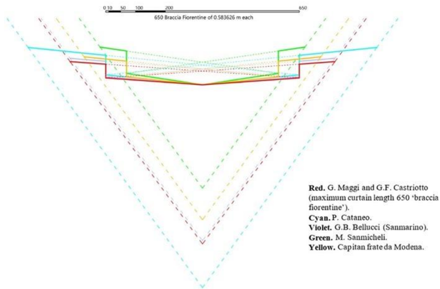
Fig. 3- Parametric configurations of the planimetric profile of fortifications following the prescriptions by Maggi and Castriotto and their references. Graphic scale in braccia fiorentine (graphic elaboration by Lorenzo Belli, 2025)
