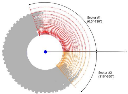
Fig. 5- Computation of missing sectors. Top view (graphic elaboration by the authors, 2025)
