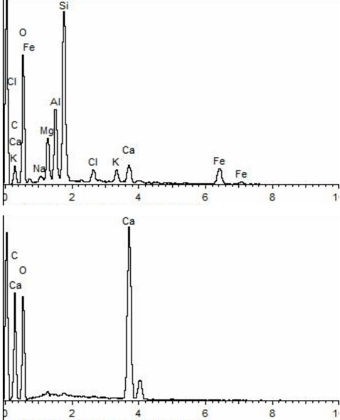
Fig. 9- Typical EDX spectrum of the aluminosilicate sand (above) and limestone aggregates (below)
