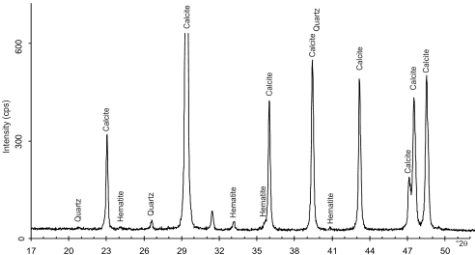
Fig. 7- XRD pattern
