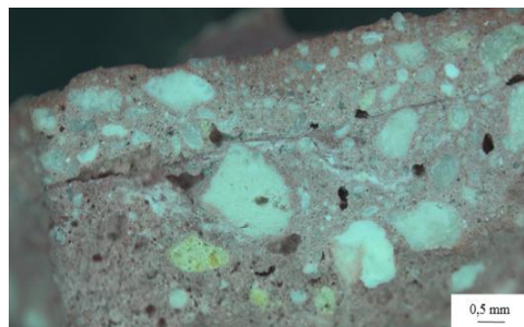
Fig. 6- Stereo-microscope image of the polished surface of the sample
