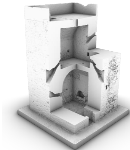
Fig. 6- Perspective view of one of the possible breakdowns of the physical model (elaboration by E. Pupi, 2025)
