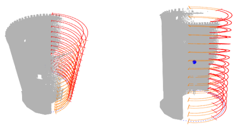
Fig. 6- Missing sectors on points cloud. Lateral views (graphic elaboration by the authors, 2025)
