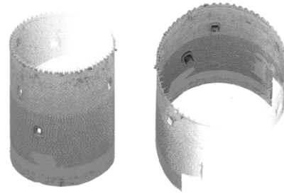
Fig. 4- Point cloud showing missing parts (graphic elaboration by the authors, 2025)
