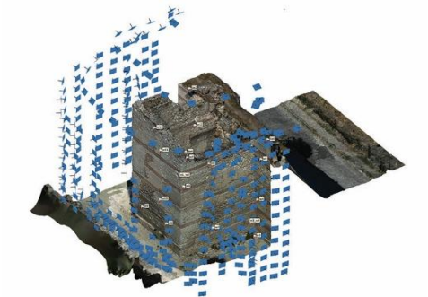
Fig. 8- Typical data acquisition and marker introduction for close-range photogrammetry: model of Tower-27 with 414 photographs (model view from the software)
